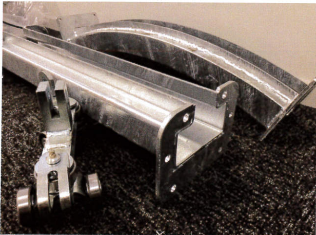
BIPLANAR & SKATE CHAIN TRACK
