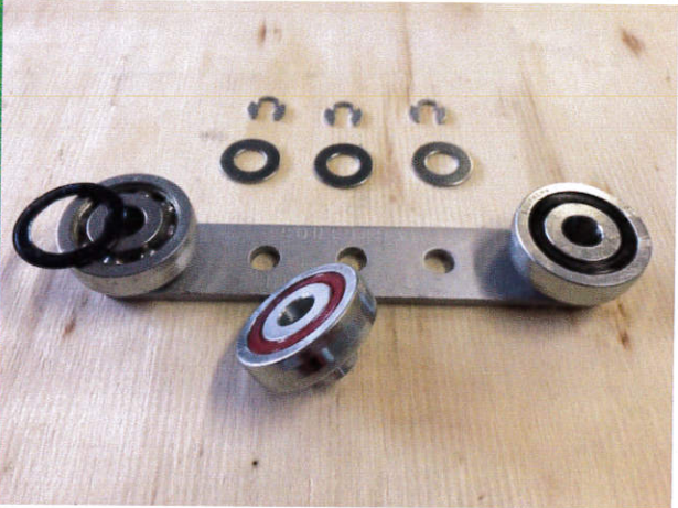
REPLACEMENT BEARINGS, CIRCLIPS & WASHERS
